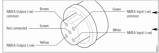
NMEA cable at Raymarine plotter
